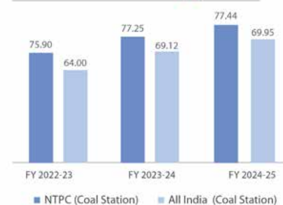
NTPC PLF Vs All India PLF (%)
